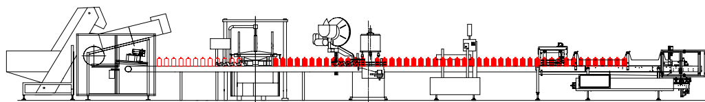
UNSCRAMBLER
